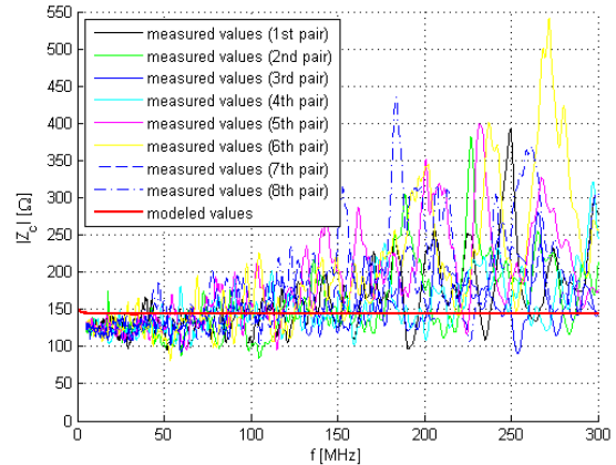
Fig. 3: Module of characteristic impedance Z_c TCEPKPFLE 75 \times 4 \times 0,4 .
