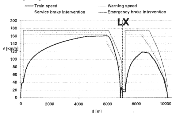
Fig.8. Distance-speed diagram of a test run on the variant "c".
