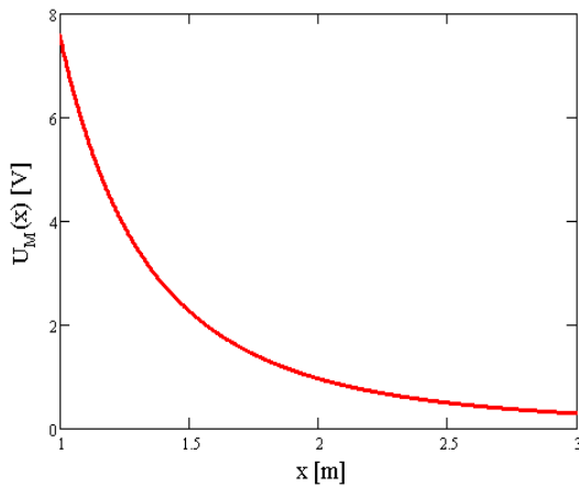
Fig. 2. Voltage induced into marker
