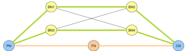
Fig. 1: An example scenario with two node-disjoint paths bypassing node FN between nodes PN and CN going through BN nodes.
